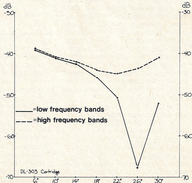
Fig. 5 — An IM distortion vs. VTA variation comparison, showing null points in the high and low frequency sections.
