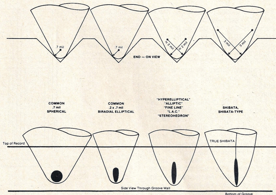
Fig. 4 — Groove contact geometry of four common stylus shapes.
